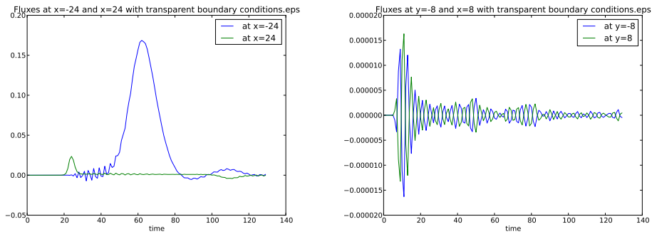
Figure 31: On the left the fluxes on the west and east boundaries and on the right the fluxes on the south and north boundaries, using transparent boundary conditions.
