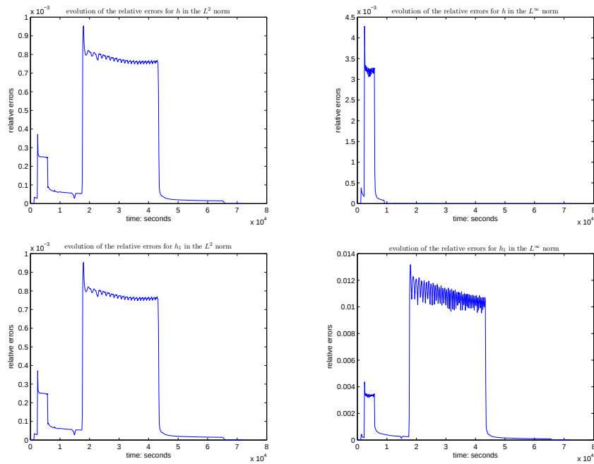
Figure 22: The evolution of the relative errors for the free surfaces h (on the top) and h_1 (on the bottom) in the case of \epsilon = -0.2 ( L^2 and L^\infty norms).
