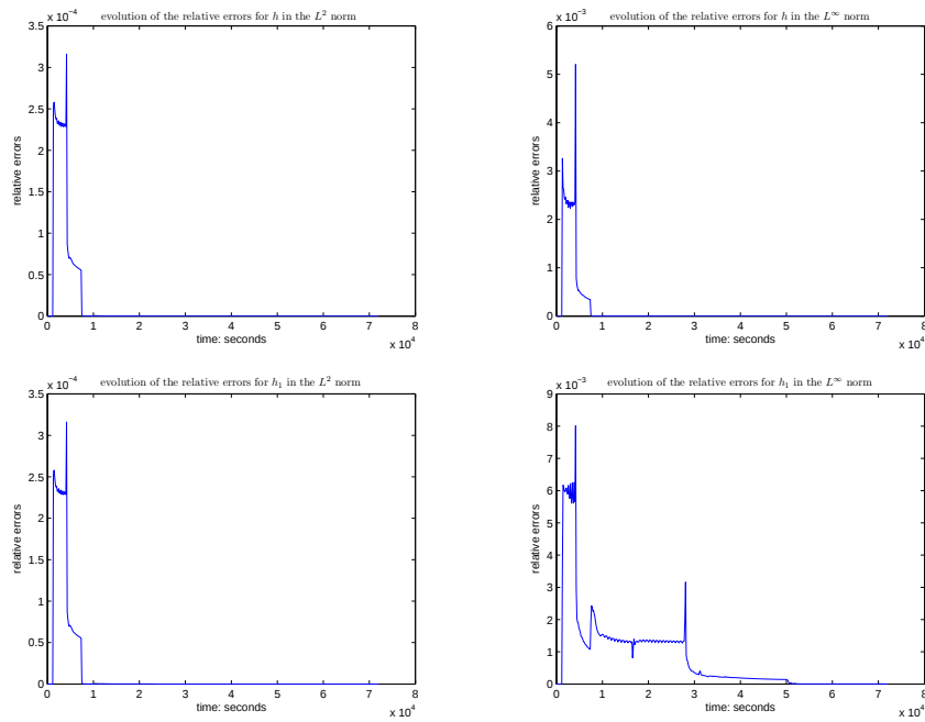
Figure 21: The evolution of the relative errors for the free surfaces h (on the top) and h_1 (on the bottom) in the case of \epsilon = 0.2 ( L^2 and L^\infty norms).
