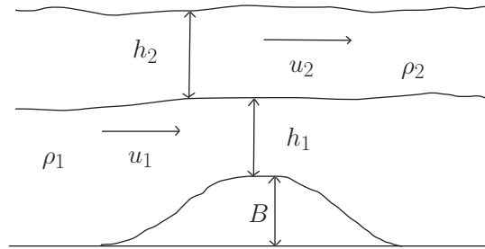
Figure 1: The two-layer shallow water model.
