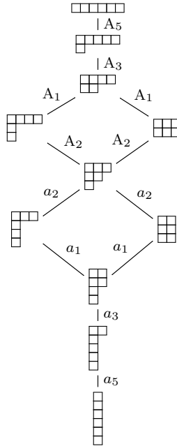
Fig. 1. Closure order on nilpotent orbits for \mathfrak{sl}_6 .
